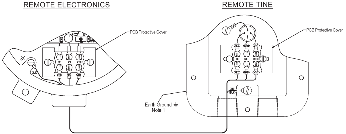
Figure 10. LP II Remote Connection Diagram
