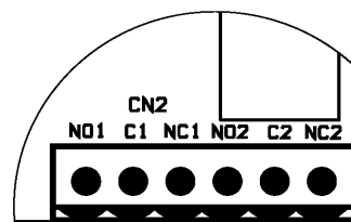
Figure 6. Main Relay Connections
